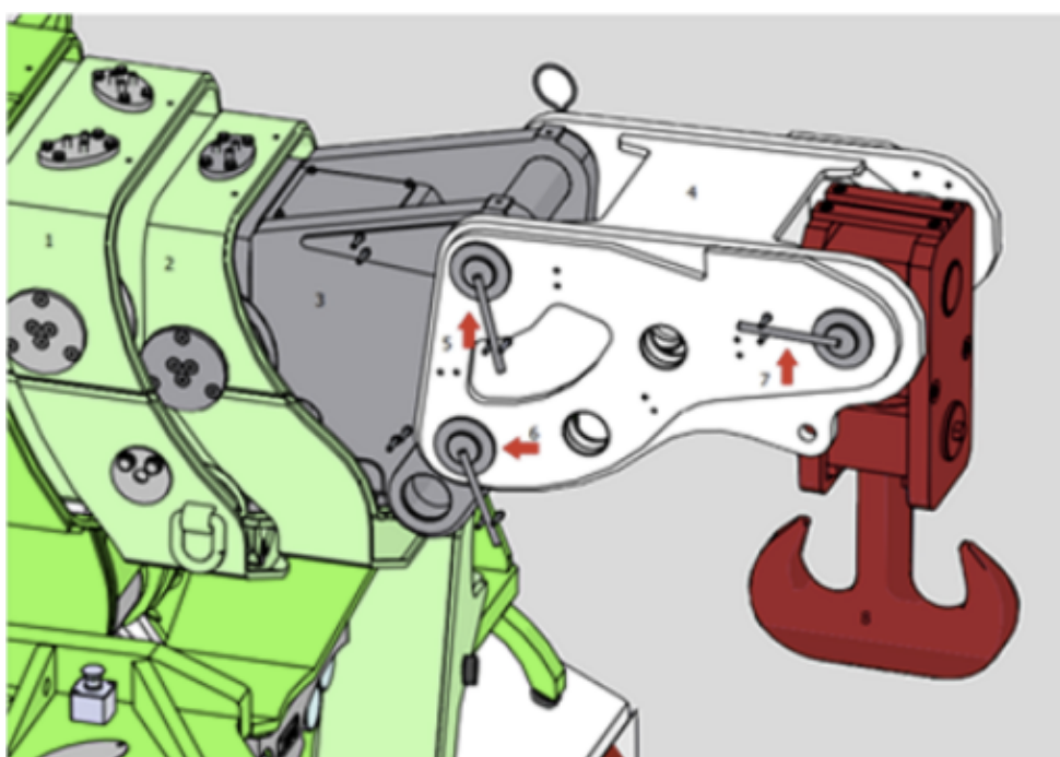
Mechanical tilting head with direct hook – load capacity 58 t
